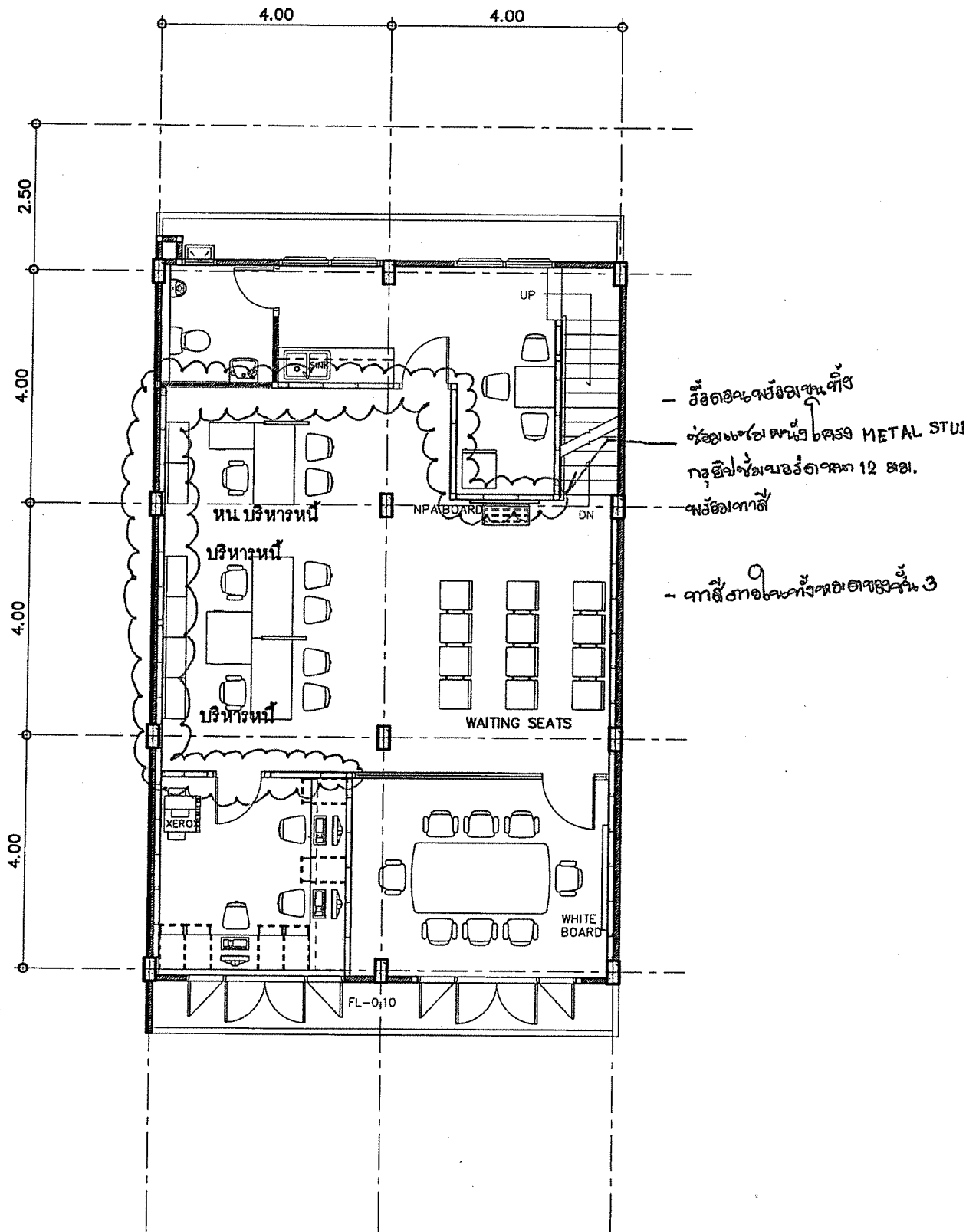
3rd.FLOOR PLAN
