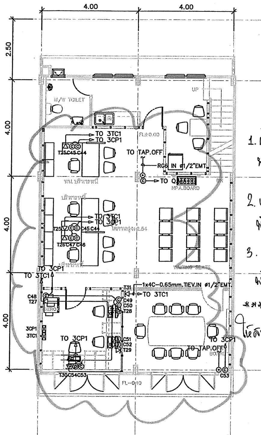
3rd. FLOOR PLAN
