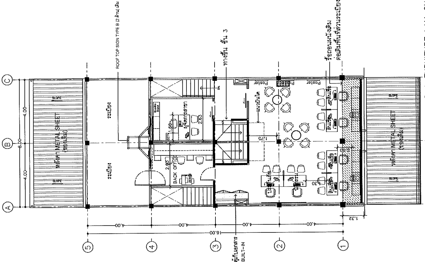
2nd. FURNITURE LAY-OUT PLAN SCALE 1:100
