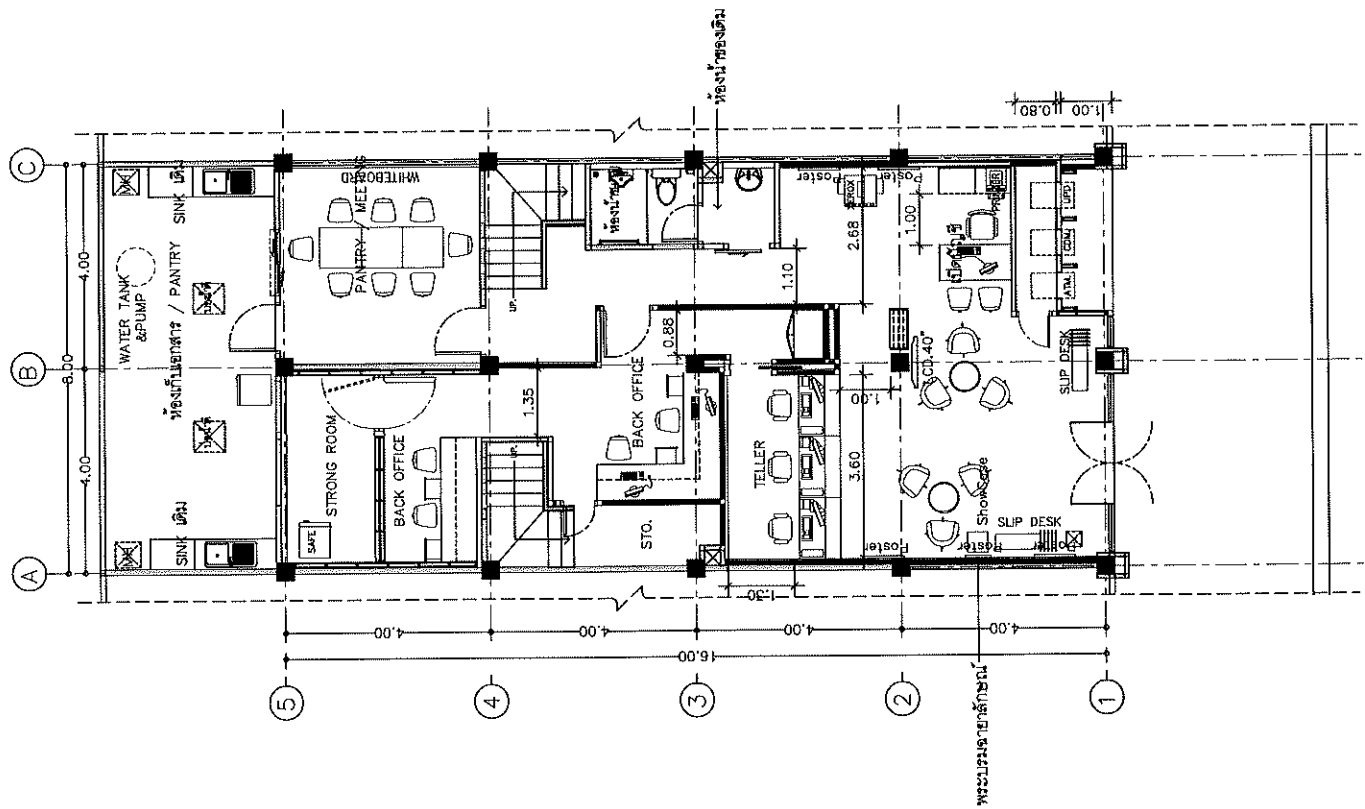
1st. FURNITURE LAY-OUT PLAN SCALE 1:100
