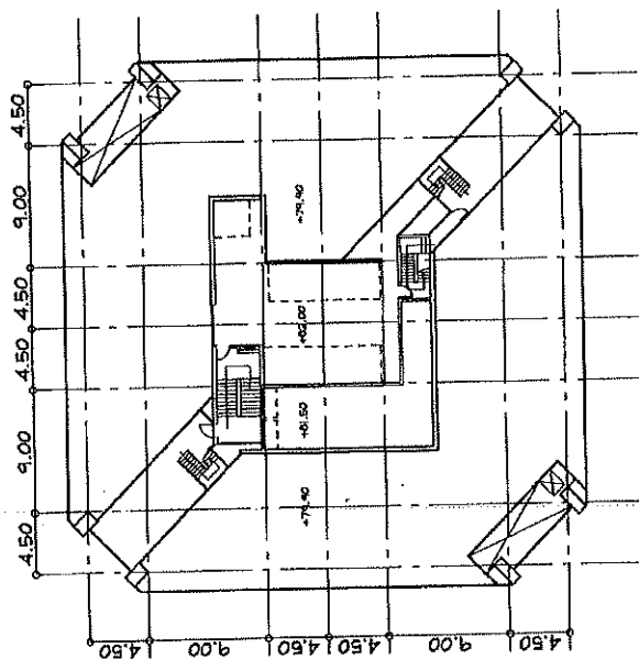
Roofing Plan SCALE 1:500
