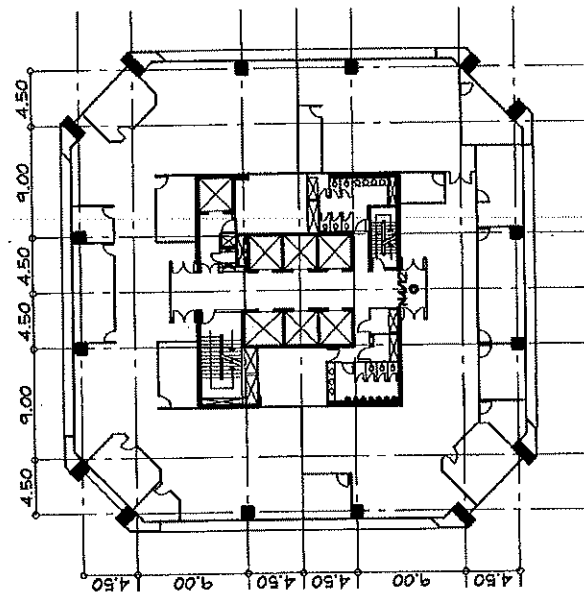
CCTV SYSTEM1 SERVICE FLOOR PLAN SCALE 1:500
