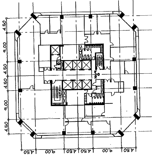
CCTV STATION 1 1/4" = 1' - 0" PLAN SCALE 1:600
