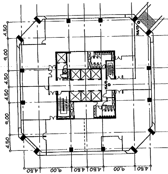
CCTV STATION 2 1/4" = 1' - 0" PLAN SCALE 1:600
