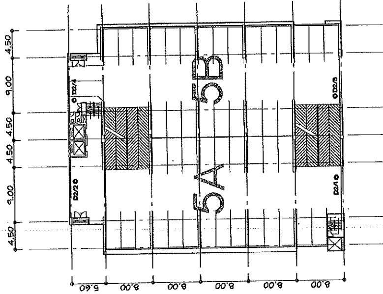
CCTV SYSTEM CANPARK 5th FLOOR PLAN SCALE 1:500
