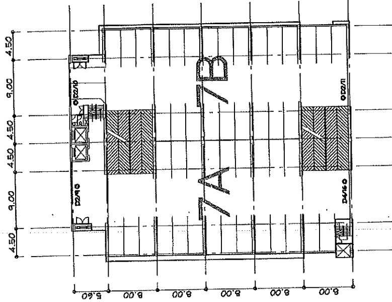
CCTV SYSTEM CAMPARK 7th Floor PLAN SCALE 1:600
