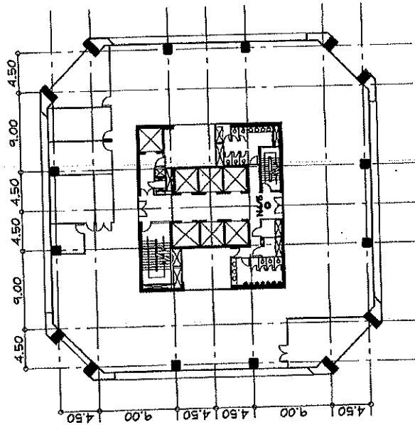
CCTV SYSTEM 9TH FLOOR PLAN SCALE 1:500
