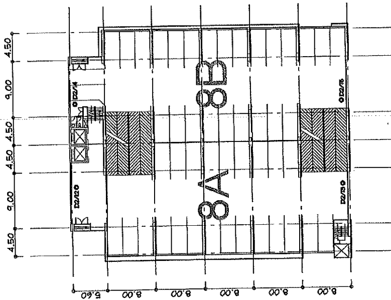
CCTV SYSTEM CAMPARK 8th Floor PLAN SCALE 1:600
