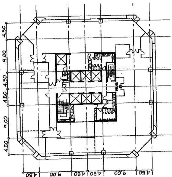
CCTV SYSTEM SERVICE FLOOR PLAN SCALE 1:500
