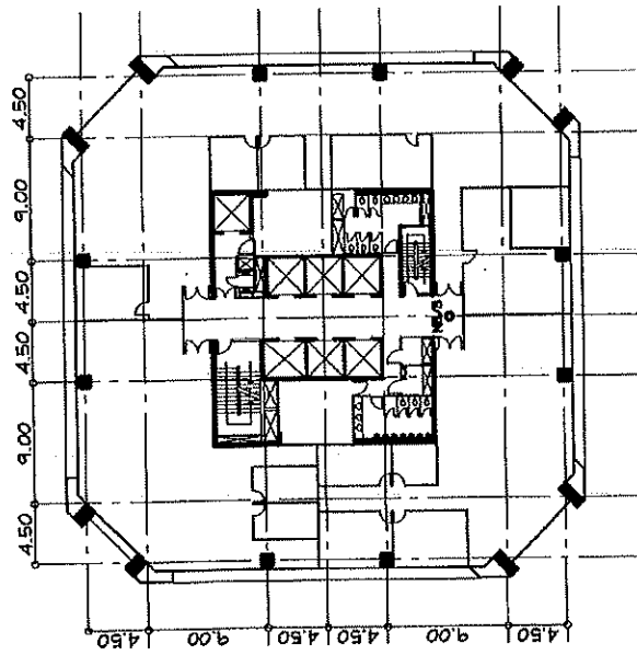
CCTV SYSTEM 1ST FLOOR PLAN SCALE 1:600
