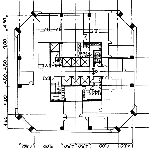
CCTV SYSTEM 8TH FLOOR PLAN SCALE 1:500
