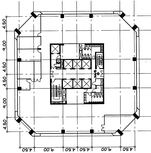
CCTV SYSTEM 9th Floor Plan SCALE 1:500
