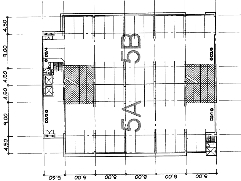
CCTV SYSTEM CAMPAK 5th Floor PLAN SCALE 1:500
