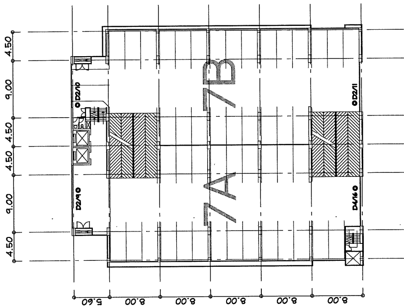
CCTV SYSTEM CAMPARK 7th Floor PLAN SCALE 1:500
