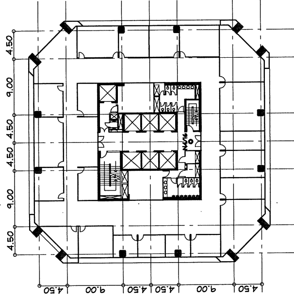
CCTV SYSTEM 1st Floor Plan SCALE 1:500
