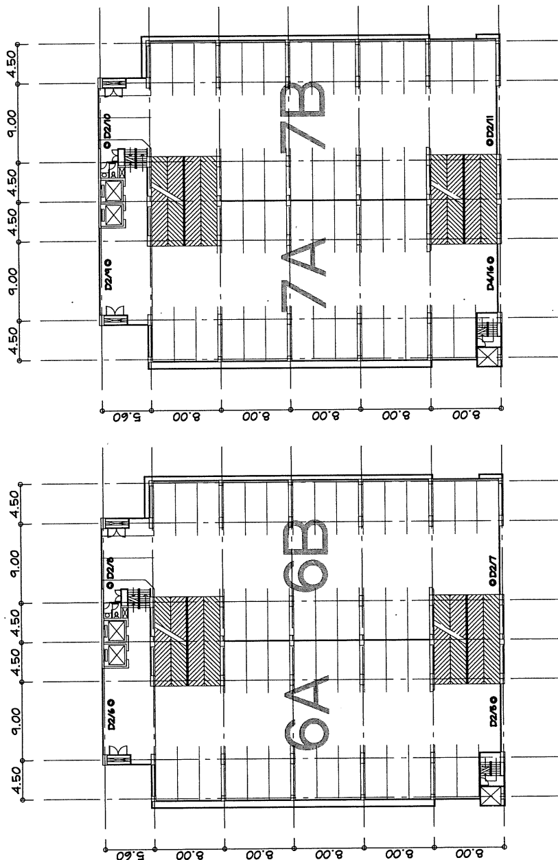
CCTV SYSTEM CAMPARK 6th Floor PLAN SCALE 1:500
