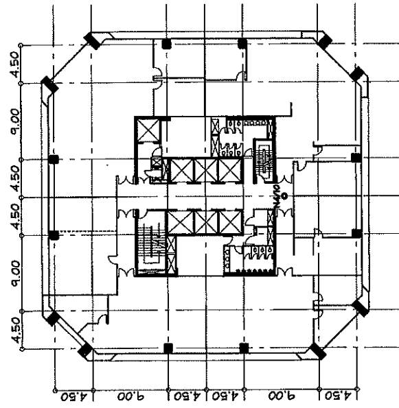
CCTV SYSTEM 19th-22 FLOOR PLAN SCALE 1:500
