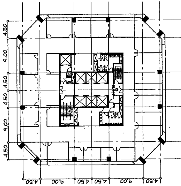
CCTV SYSTEM 18TH FLOOR PLAN SCALE 1:500
