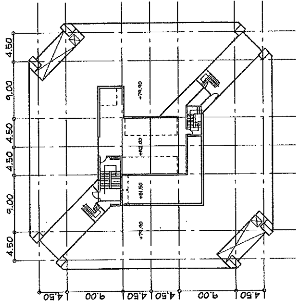
Roof Plan SCALE 1:500
