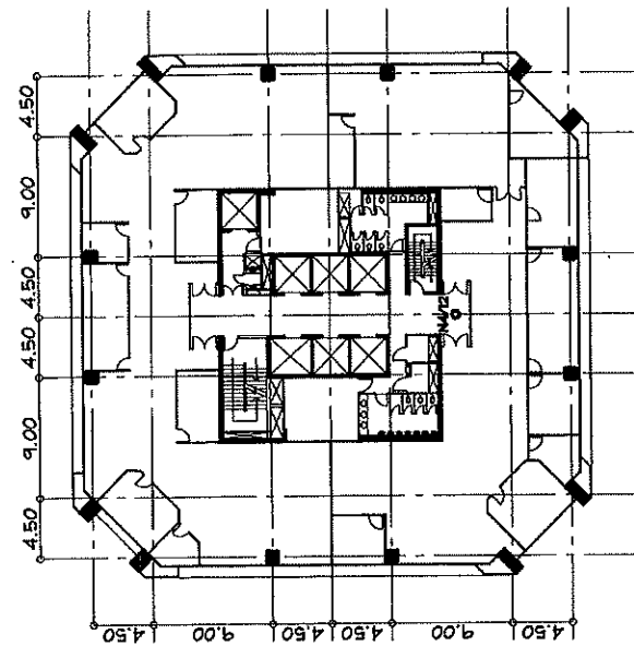
CCTV SYSTEM 1982 FIRST PLAN SCALE 1:500
