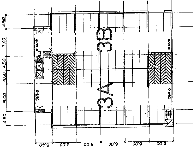
CCTV SYSTEM CAMPARK 2nd Floor PLAN SCALE 1:600
