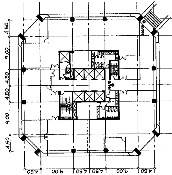
CCTV SYSTEM 5TH FLOOR PLAN SCALE 1:600
