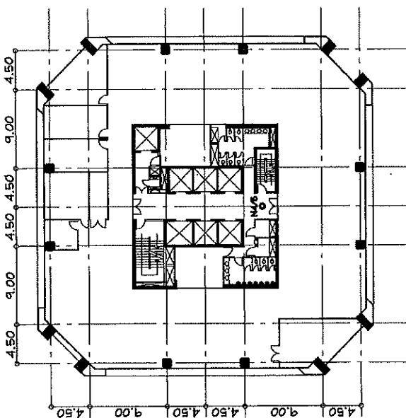
CCTV SYSTEM BRIDGE FLOOR PLAN SCALE 1:500
