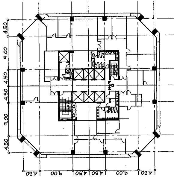
CCTV SYSTEM 4TH FLOOR PLAN SCALE 1:600
