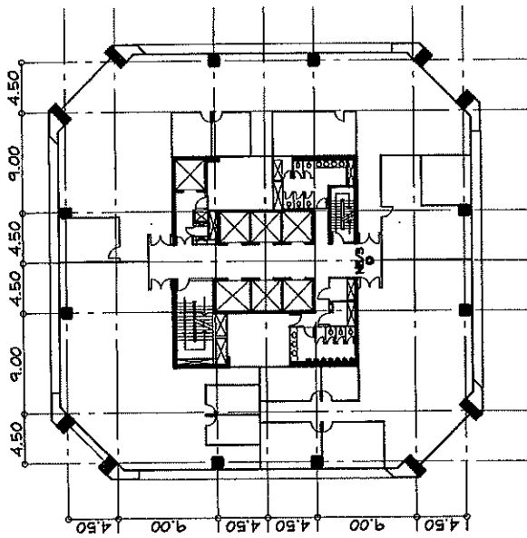
CCTV SYSTEM 1 3RD FLOOR PLAN SCALE 1:500
