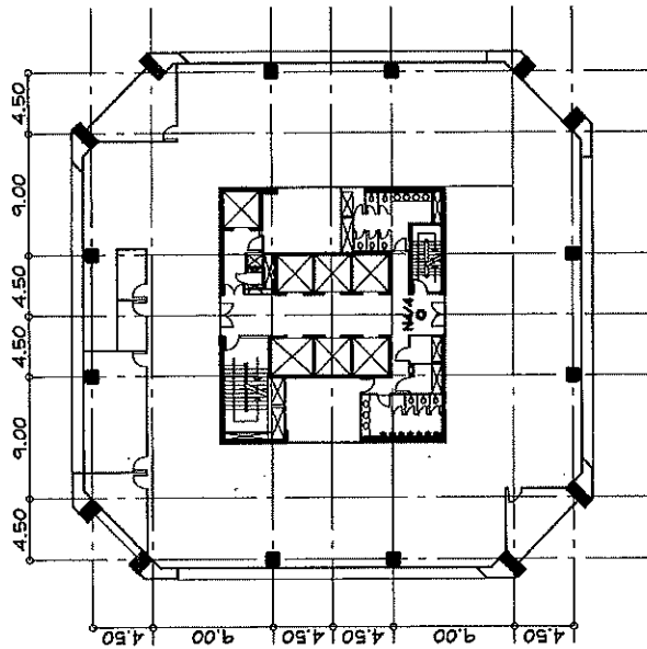
CCTV SYSTEM BRIDGE FLOOR PLAN SCALE 1:500
